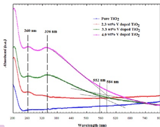
21 Figure 2 UV-Vis spectra of undoped TiO 2 and M-V doped TiO 2 at 2.3, 3.3 and 4.9 wt% V doped TiO 2 suspended in ethanol solution.
